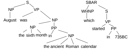
Figure 2: Segmentation
