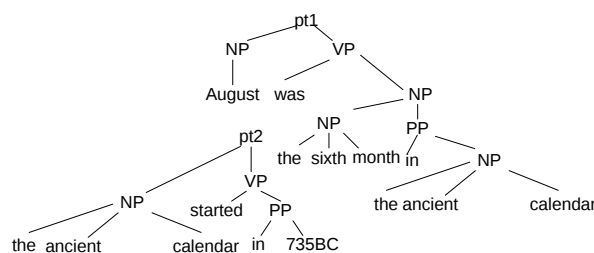
Figure 4: Dropping & Reordering
