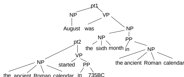
Figure 3: Completion
