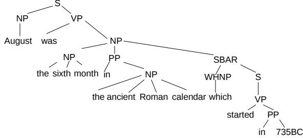
Figure 1: Parse Tree of c
